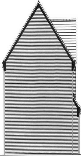
SIDE ELEVATION
