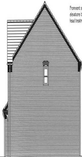
SIDE ELEVATION
